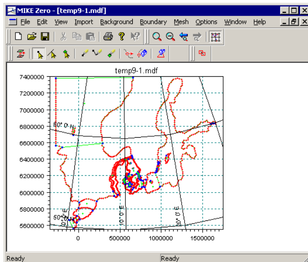
The Mesh Generator is an efficient MIKE Zero tool for the generation and handling of unstructured meshes, including the definition and editing of boundaries
